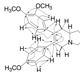
Figure 2. Selected HMBC connectivities observed for 3 . The experiment was optimized for ^nJ_{\text{C,H}} = 7 Hz.
